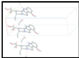
Fig. 2. Part of the crystal structure of the title compound, showing the formation of a C(7) chain, along [100]. H atoms not involved in this motif were omitted for the sake of clarity.
